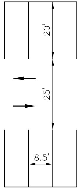
90° PARKING DETAIL SCALE: 1"=20'
