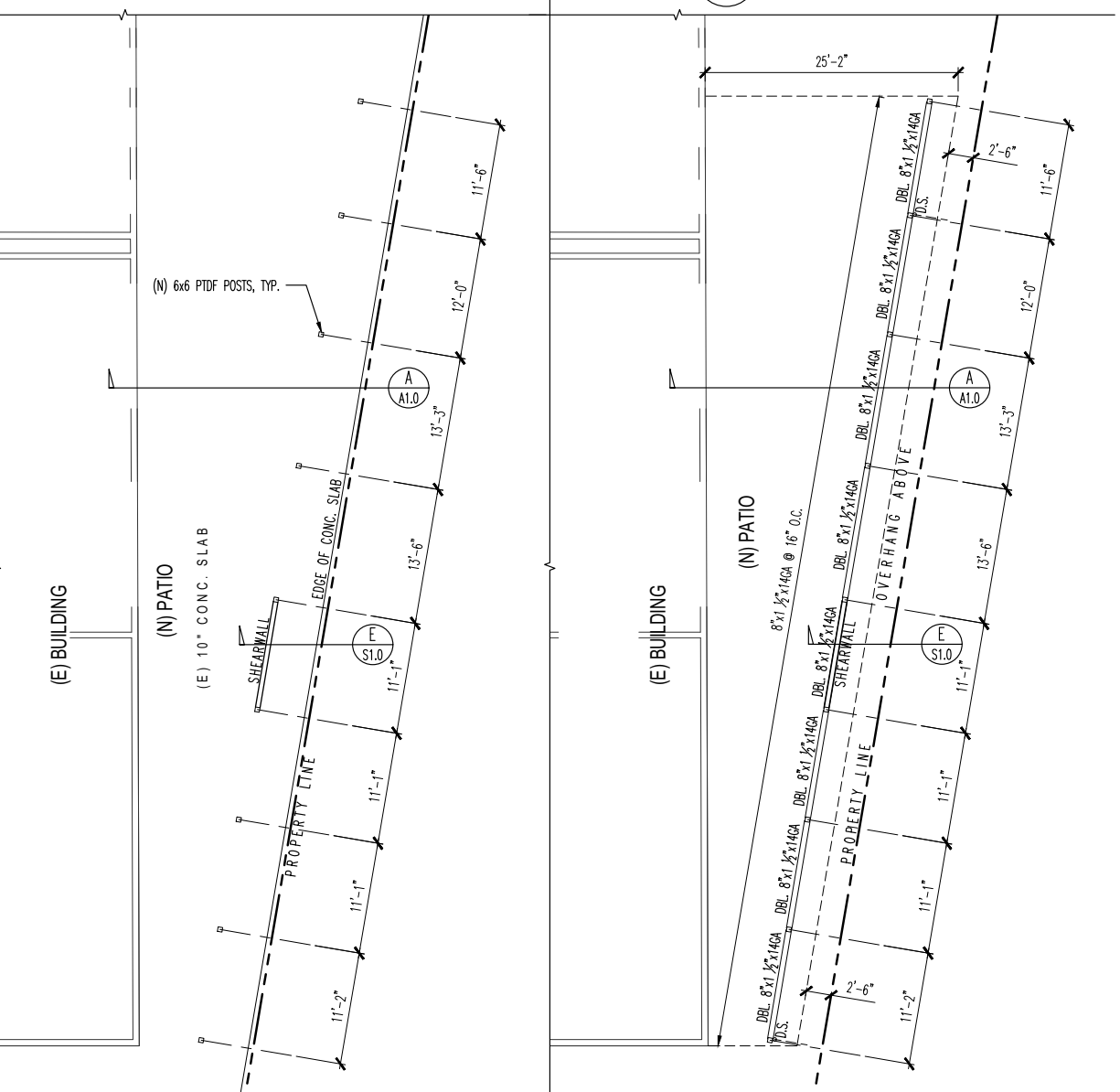
FOUNDATION PLAN Scale 1/8" = 1'-0"
