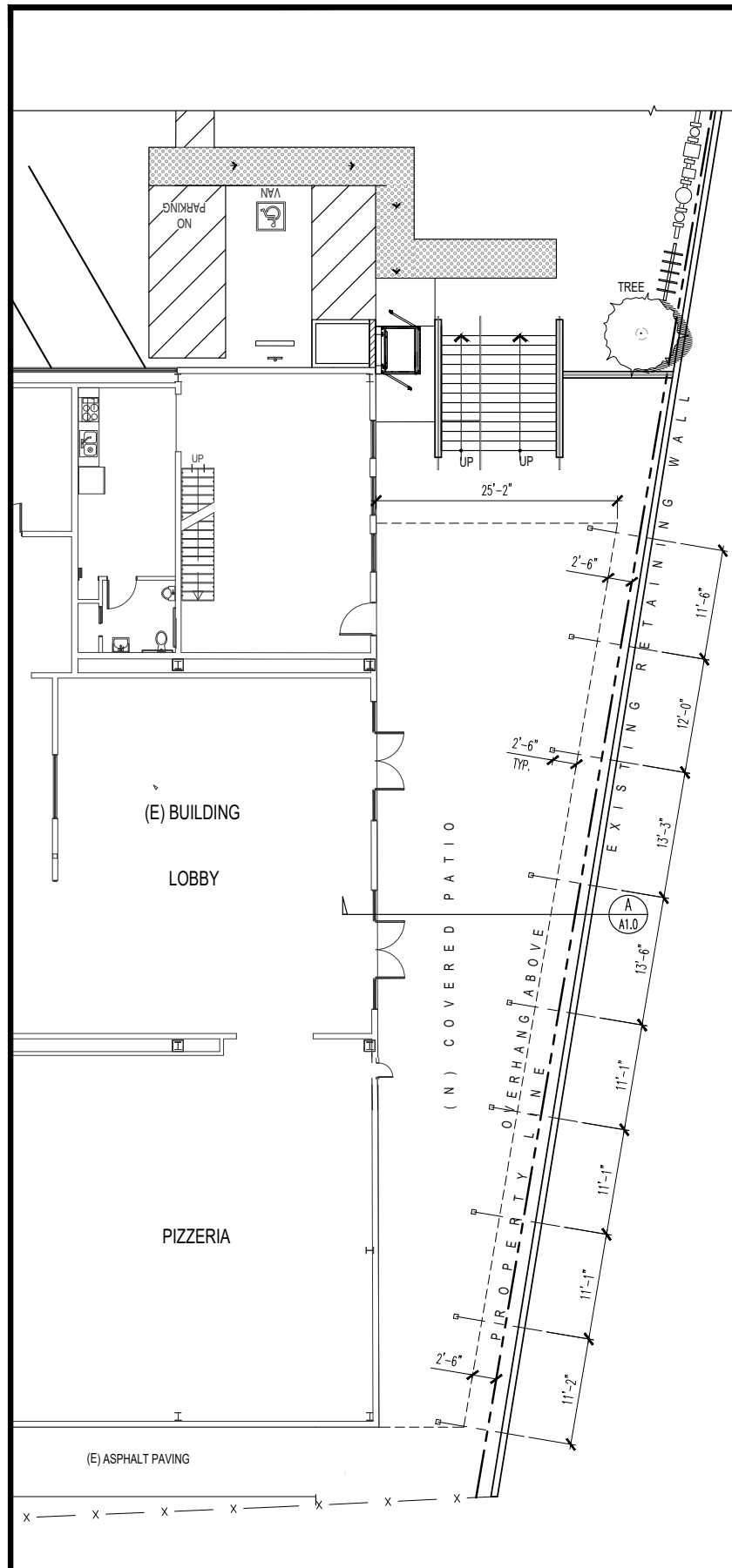
COVERED PATIO PLAN Scale 1/8" = 1'-0"
