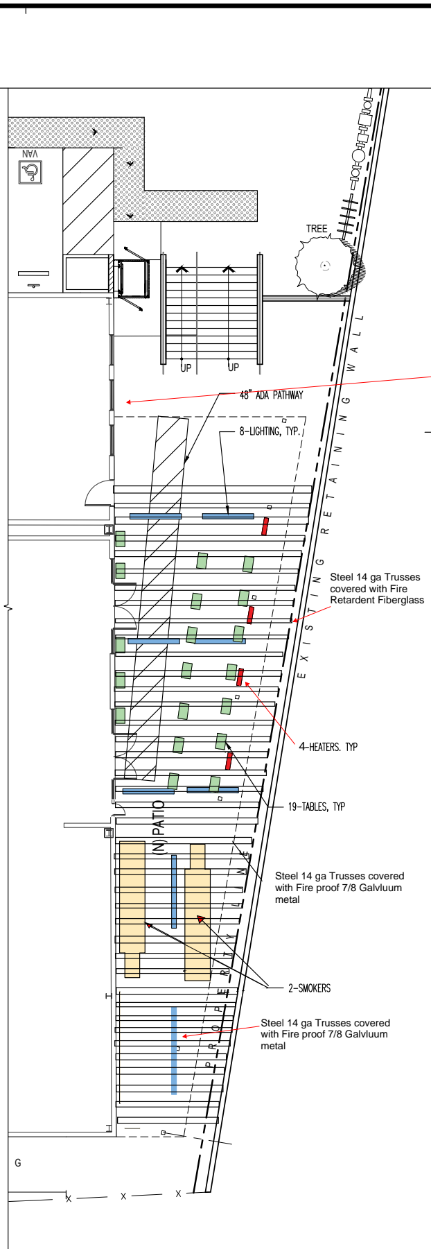
TENANT IMPROVEMENT PLAN Scale 1/8" = 1'-0"
