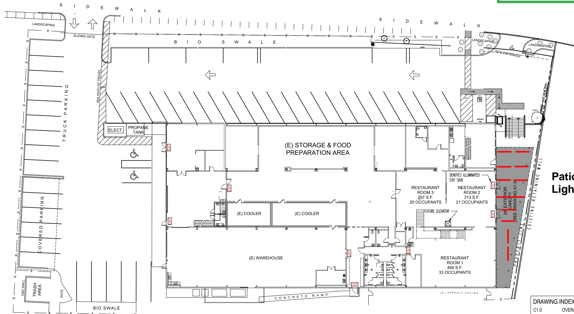
OVERALL SITE PLAN Scale 1/8" = 1'-0"
