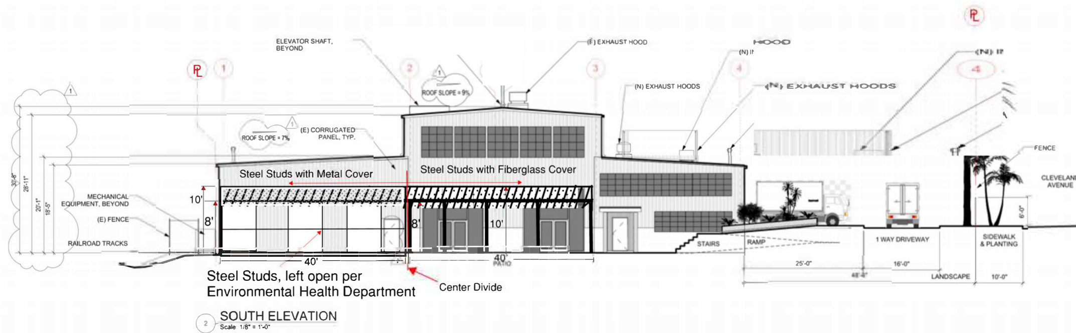
Fiberglass Cover over seating area
