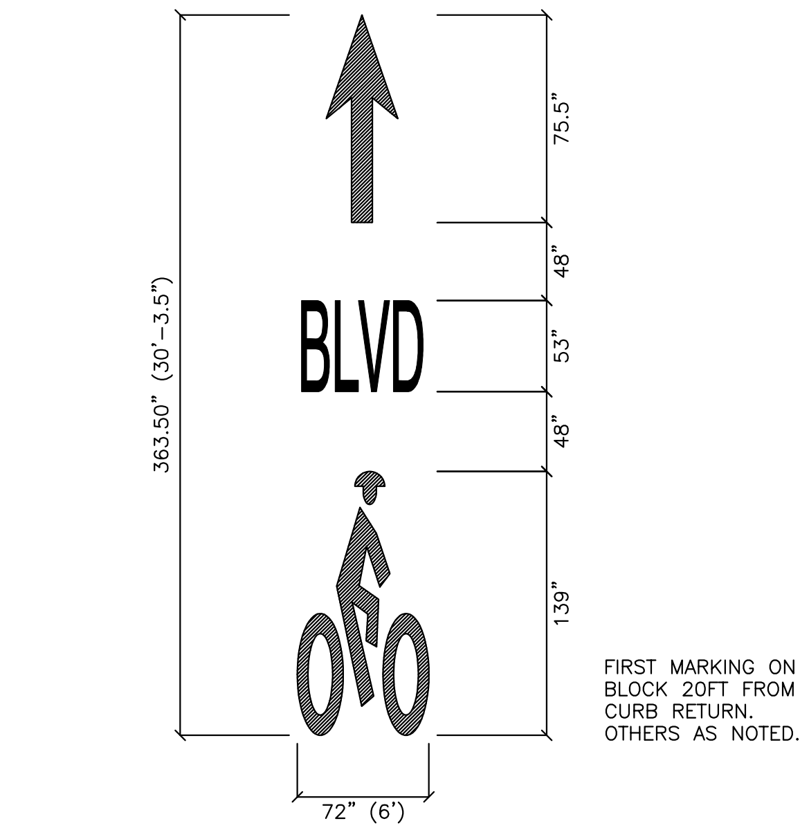
DETAIL 'C' BIKE BOULEVARD MARKING DETAIL N.T.S.
