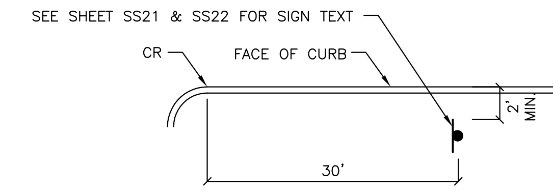
DETAIL 'E' TYPICAL GUIDE SIGN INSTALLATION LAYOUT N.T.S.
