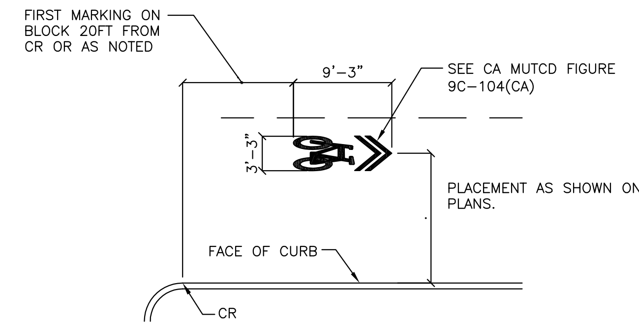
DETAIL 'A' SHARED ROADWAY BICYCLE MARKING N.T.S.
