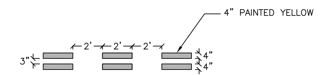
DETAIL 'H' MODIFIED DETAIL 21 N.T.S.
