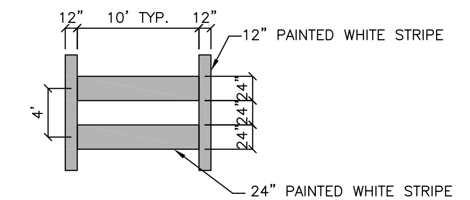
DETAIL 'G' CROSSWALK DETAIL N.T.S.
