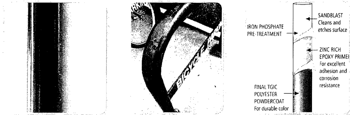
Figure 2-3: Powder coat (photos: Dero Bike Racks; Andrew J. Besold; figure: Dero Bike Racks)
