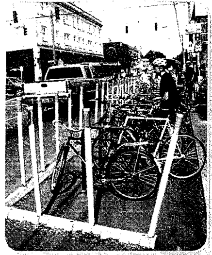
Figure 2-41: In-street bicycle parking with flexible bollards in Portland, Ore. (photo: Eric Anderson)
