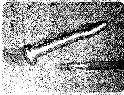
Figure 2-16: Tamper-proof anchor for flange mounting or securing rail-mounted racks (photo: John Ciccarelli)
