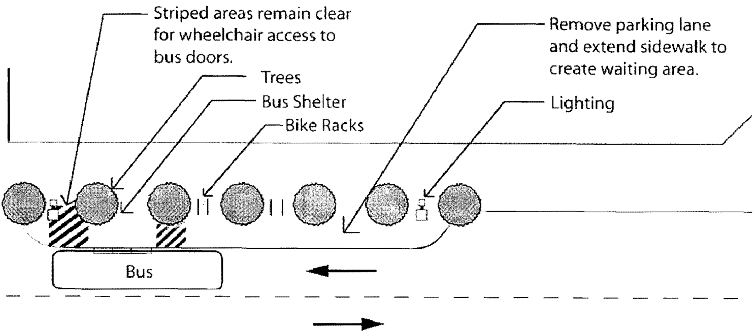
Figure 2-24: Sample ADA-compliant sidewalk rack site plan in bus stop area
