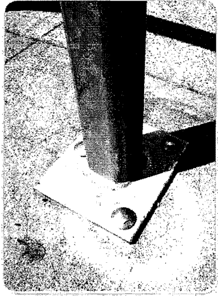
Figure 2-14: Flange concrete rack mounting (photo: Eric Anderson)
