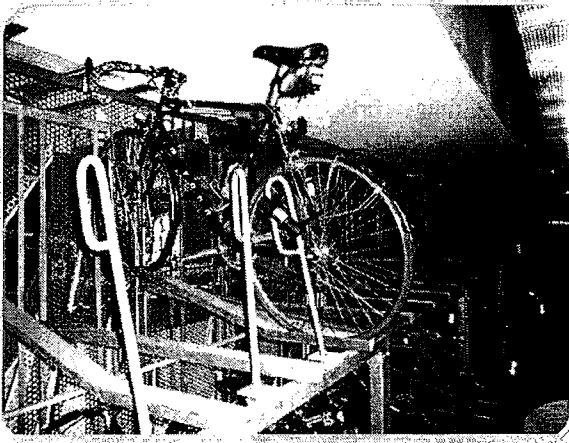
Figure 2-7: Swiveling locking arm (photo: John Ciccarelli)
