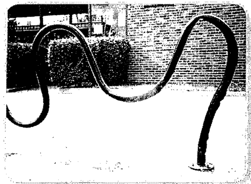
Figure 2-47: Damaged bicycle rack; Chicago, Ill. (photo: Eric Anderson)
