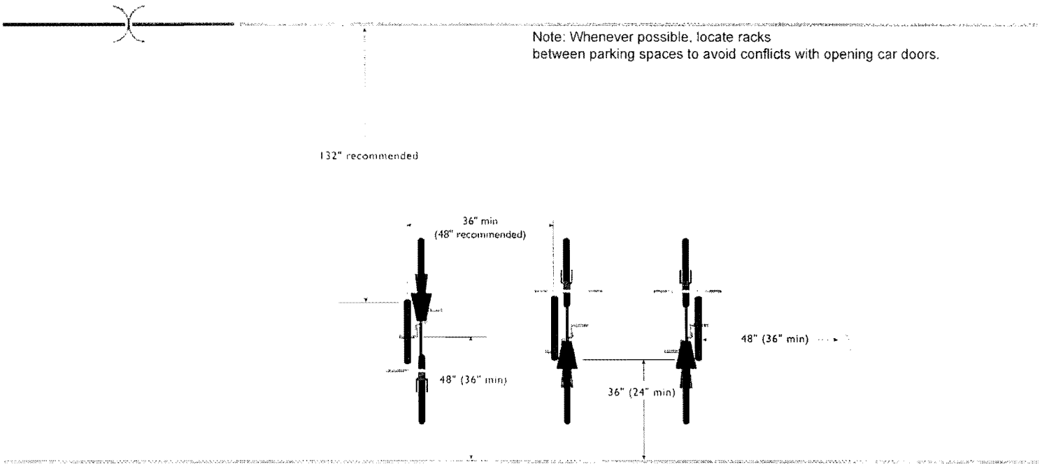
Figure 2-23: Sample layout, racks perpendicular to curb
