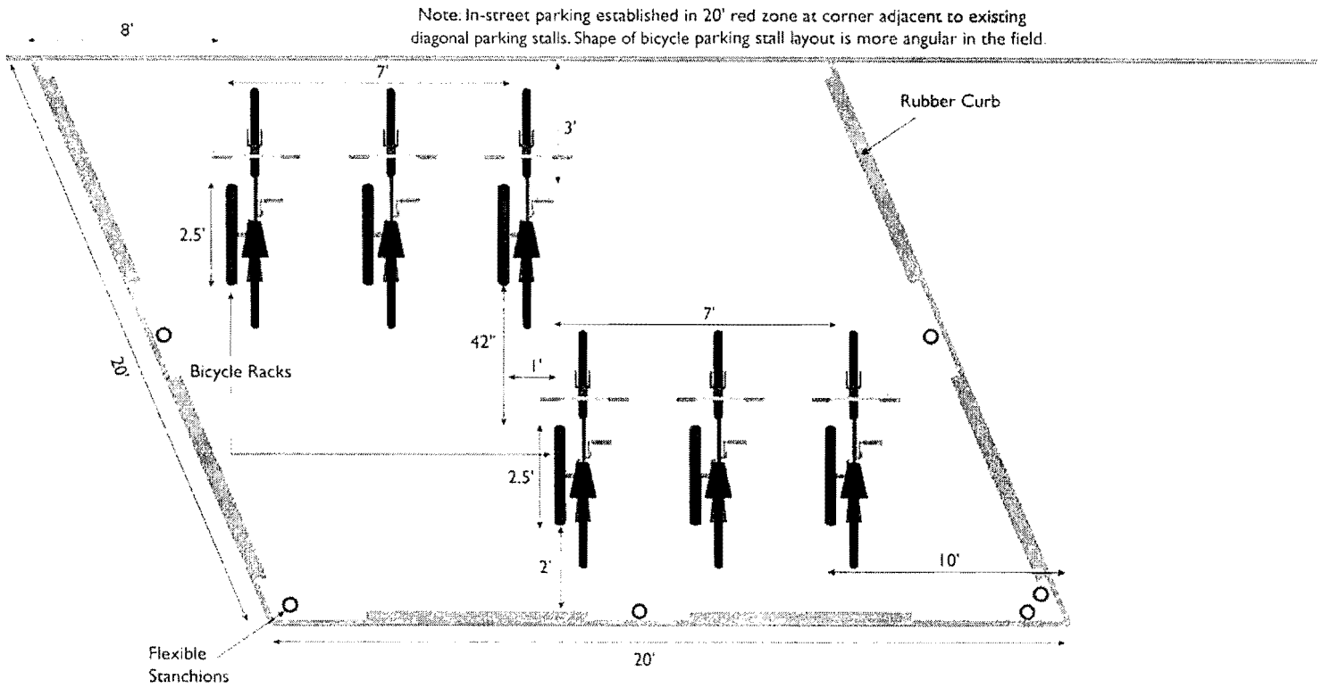
Figure 2-45: Sample in street diagonal parking stall layout, City of Berkeley, Calif.
