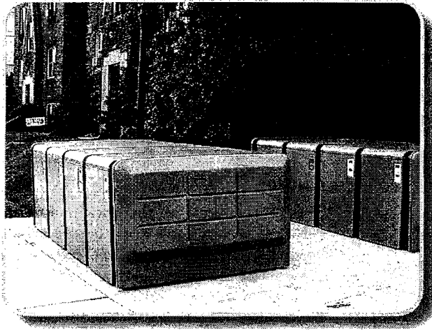
Figure 2-11: Fiberglass panel locker (photo: CycleSafe, Inc.)
